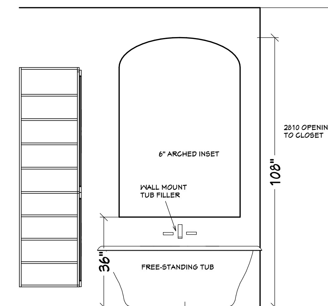
Elevation 18 scale 1/2"=1'-0"
