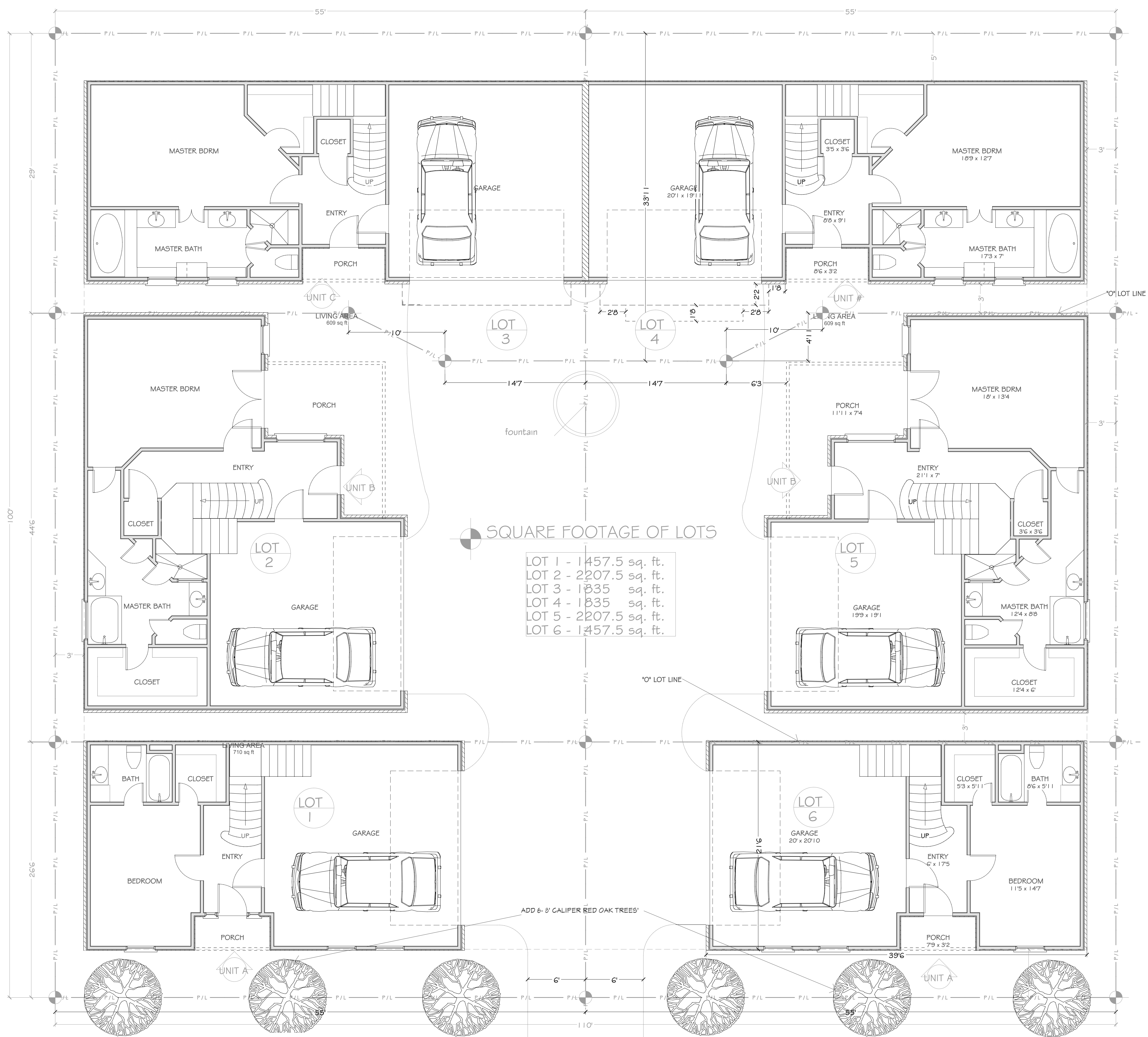
SITE PLAN 3/16" = 1'-0"
